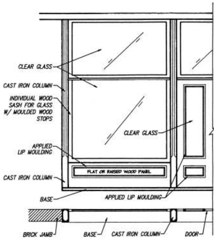
STOREFRONT DETAIL FIGURE 11
