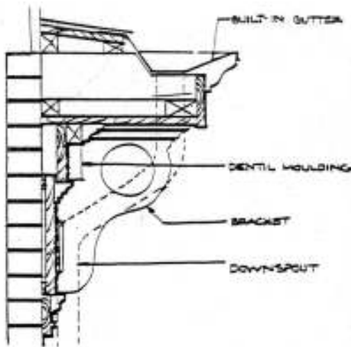
CORNICE DETAIL FIGURE 5
