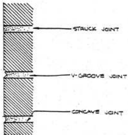
TYPICAL MASONRY JOINTS MORTAR JOINTS FIGURE 8
