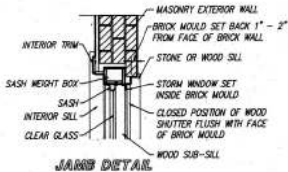
EXTERIOR STORM WINDOW FIGURE 15
