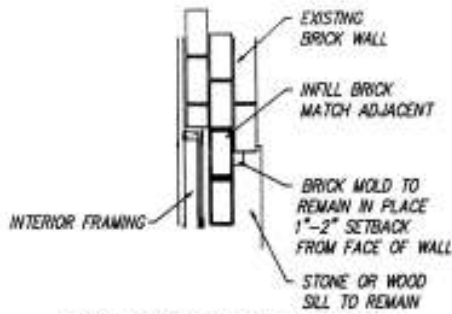
WINDOW HEAD SECTION
