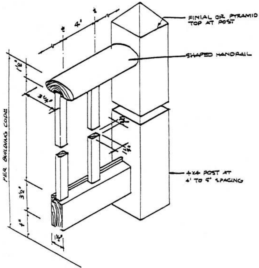
SOULARD RAIL FIGURE 18
