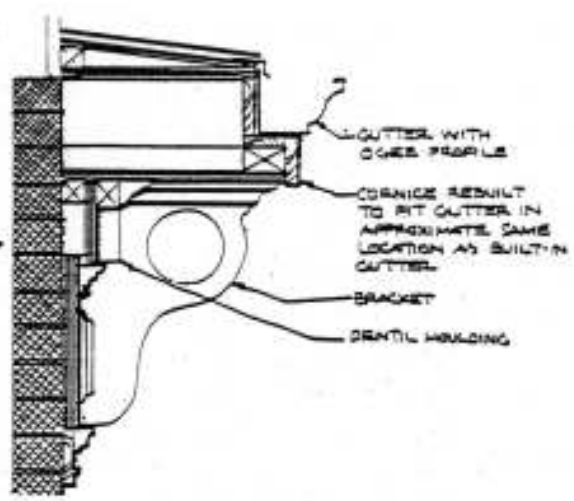
CORNICE DETAIL FIGURE 6
