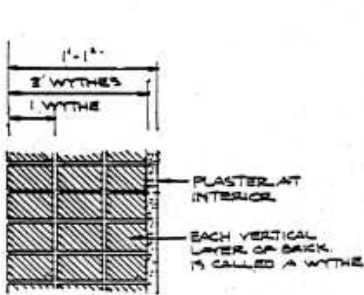
3 WYTHE WALL FIGURE 7
