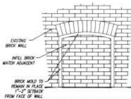
WINDOW HEAD ELEVATION BRICK INFILL OF EXISTING WINDOW OPENING FIGURE 16
