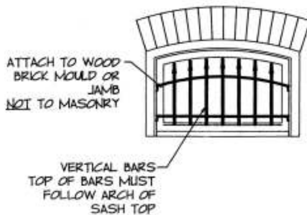
IRON ELEMENTS FIGURE 19
