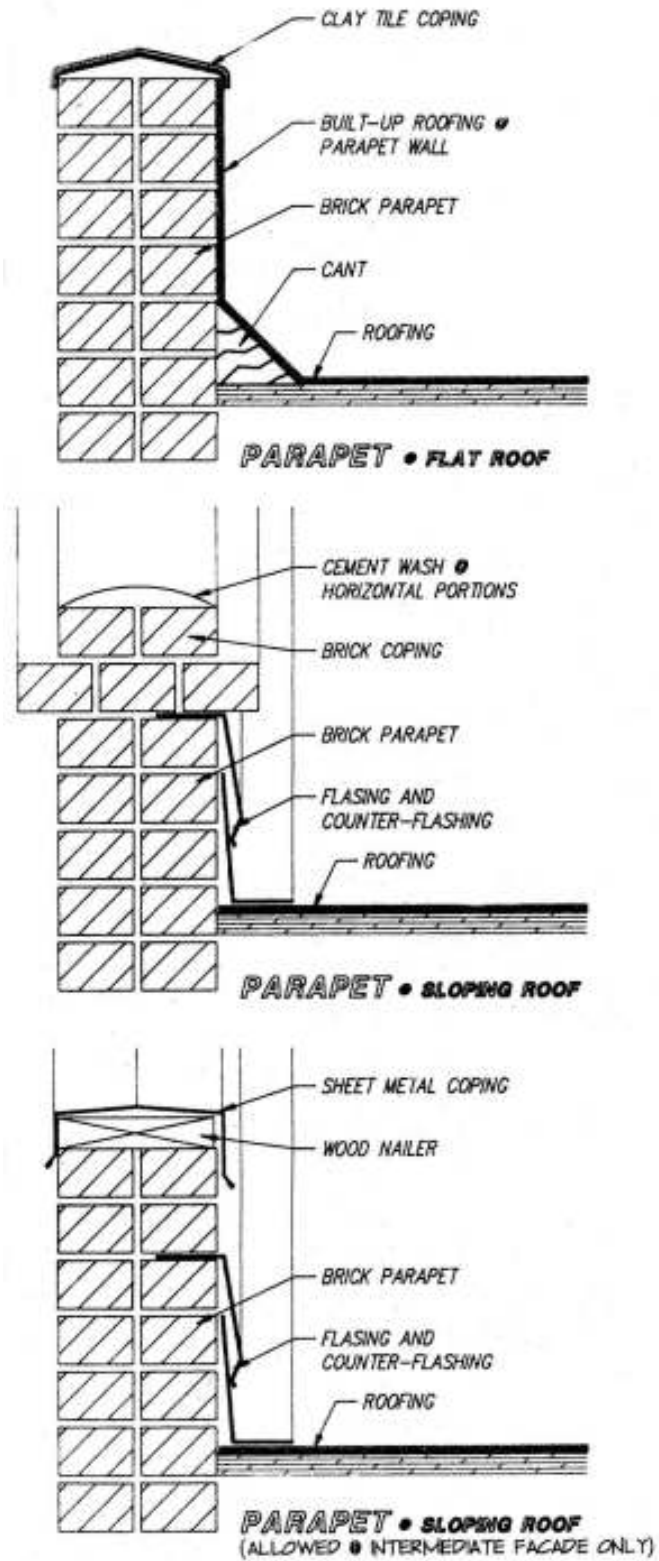
PARAPETS FIGURE 4
