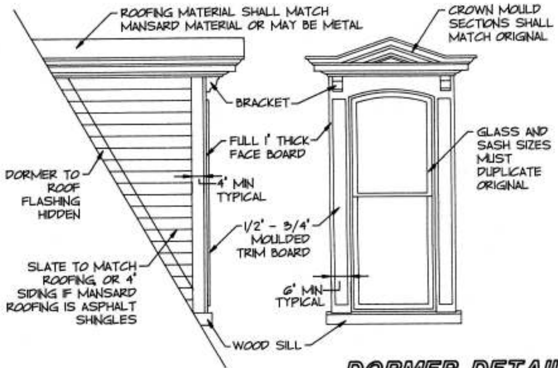
DORMER DETAIL FIGURE 20
