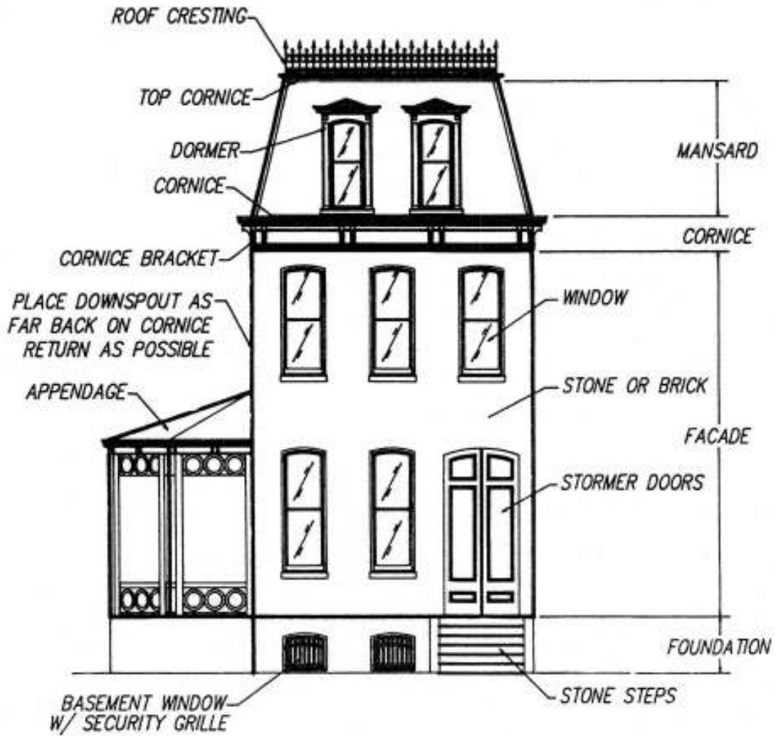
PUBLIC FACADE 2ND EMPIRE TOWNHOUSE FIGURE 1
