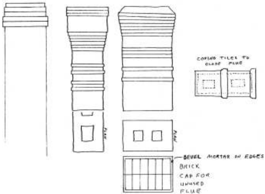
CHIMNEY TOPS FIGURE 12
